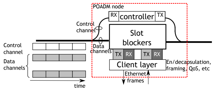
Fig. 1. Optical slot switching POADM node description.
