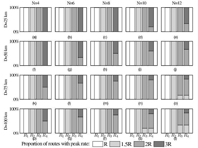
Fig. 2. Distribution of the maximum usable rates across all network routes, assuming uniform traffic demand over all pairs of network nodes; each subfigure corresponds to a different network sizes ( N, D ); each bar corresponds to a set of available rates: \mathcal{R}_1, \mathcal{R}_2, \mathcal{R}_3 , or \mathcal{R}_4 .
