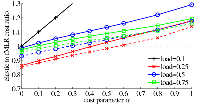
Fig. 6. Cost of elastic vs. fMLR networks for N=10 nodes, D=100 km, 3 rates ( \mathcal{R} = \mathcal{R}_3 ). Plain lines: uniform traffic, dashed lines: gravity traffic.
