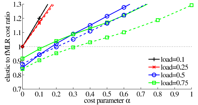
Fig. 3. Cost of elastic vs. fMLR networks for N=6 nodes, D=50 km, 4 rates ( \mathcal{R} = \mathcal{R}_4 ). Plain lines: uniform traffic, dashed lines: gravity traffic. There is no difference between uniform and gravity cost ratios for load=0.1.
