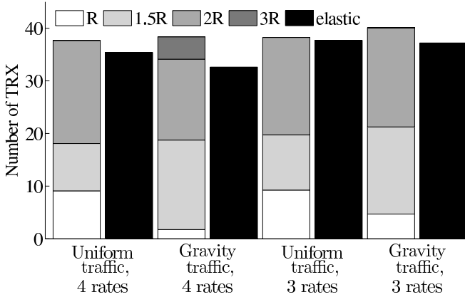
Fig. 5. Number of transponders ( N=10 nodes, D=100 km) when the number of available rates is either 3 or 4, for cost factor \alpha=0.2 .
