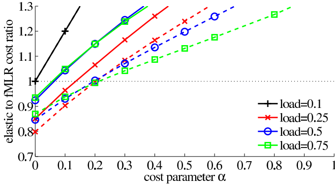
Fig. 4. Cost of elastic vs. fMLR networks for N=10 nodes, D=100 km, 4 rates ( \mathcal{R} = \mathcal{R}_4 ). Plain lines: uniform traffic, dashed lines: gravity traffic.
