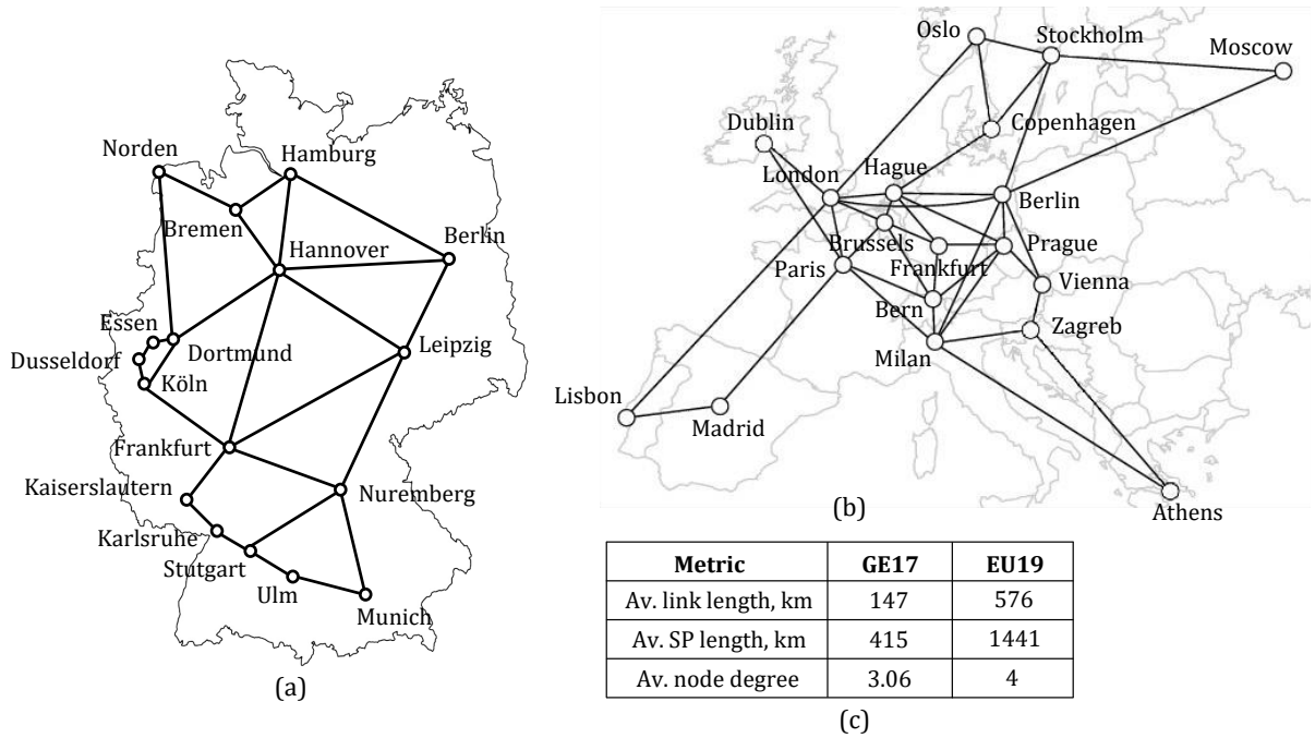
Fig. 5. (a) 17-node German and (b) 19-node European topologies (c) Topology parameters
