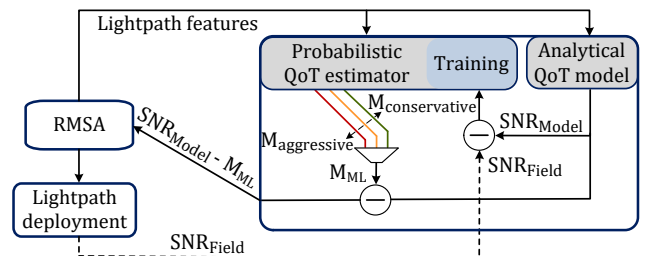
Fig. 4. Proposed probabilistic QoT estimator integrated into Routing, Modulation format selection and Spectrum Allocation (RMSA) procedure
